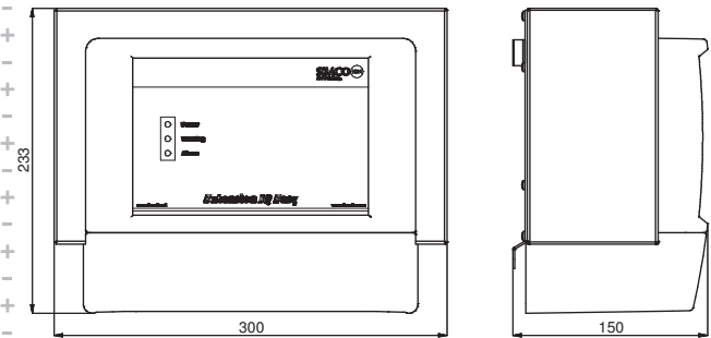
Technical drawing Extension IQ Easy
