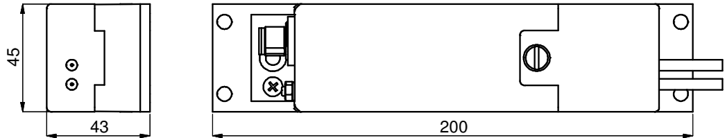
Technical drawing CMME
